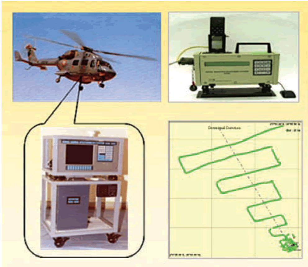
Aerial Gamma Spectrometry System
